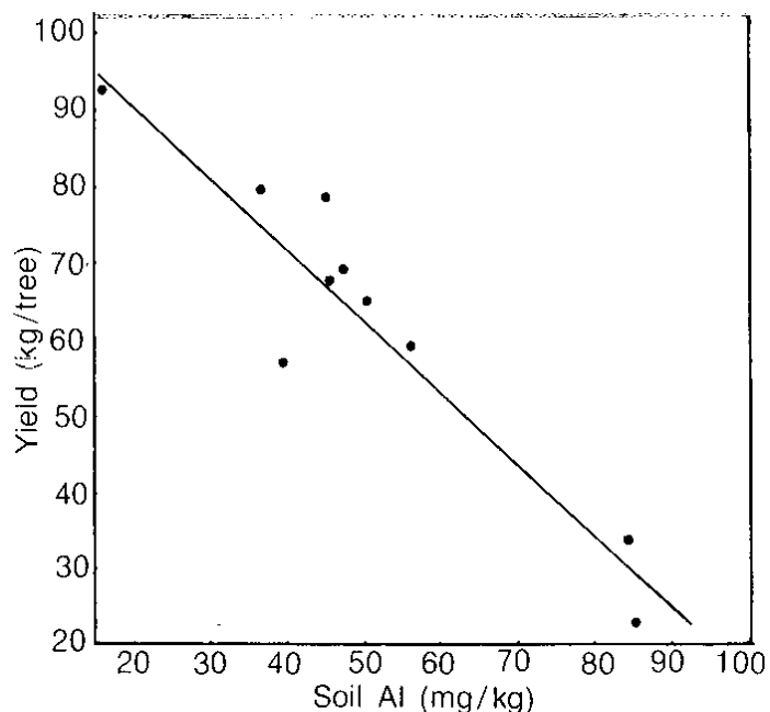
Fig 1 The relationship between topsoil Al concentration and yield 1983/84 season, mean values per treatment ( r = -0,94 and y = 108,93 - 0,932x ).
