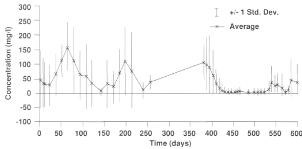
Fig. 1. Nitrate-N in soil water 80% ET c treatment.
