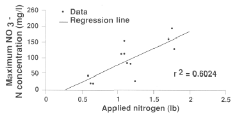
Fig. 3. Effect of applied nitrogen on maximum nitrate-N.
